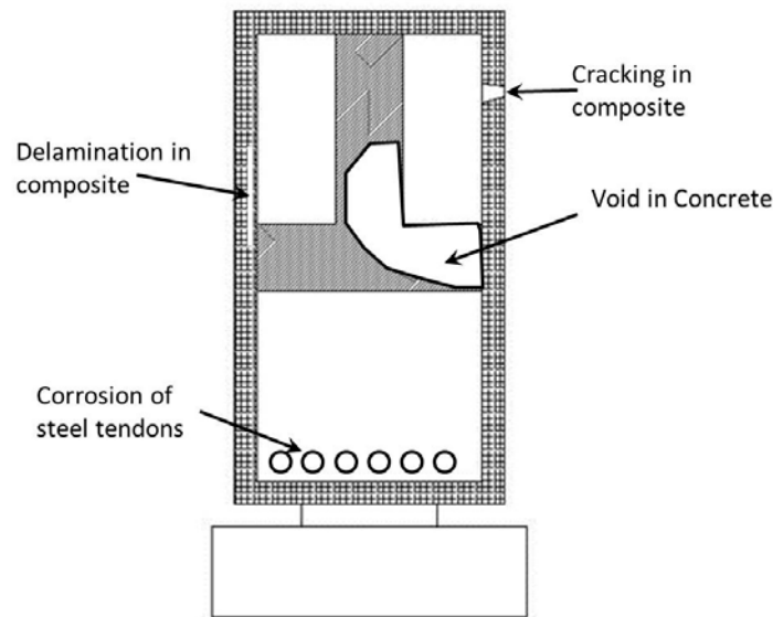
Figure 4-1 Example of Potential Damage Modes for HCB
