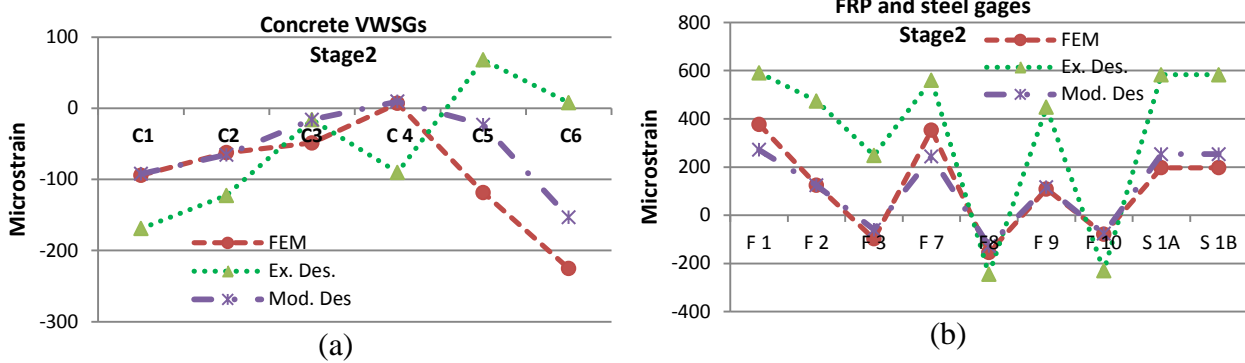
Figure 6-8 Strain Values in HCB2, B0410, Due to the Deck Pour (Stage 2)
