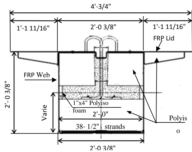
Figure 3-12 Typical Cross Section of B0478 HCB
