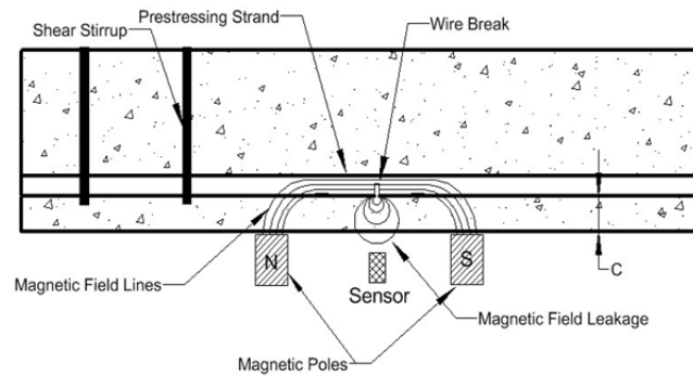
Figure 4-4 Magnetic Flux Leakage Test Schematic
