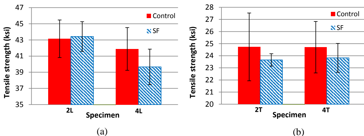
Figure 7-8 Tensile Strength of Control and Salt Fog
