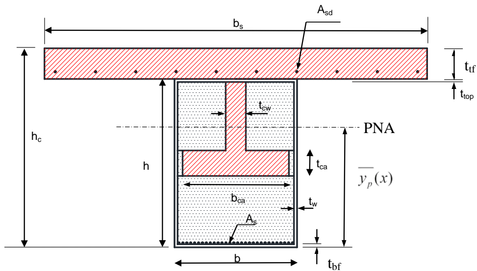
Figure 6-5 Typical Cross-section of the Composite Hybrid-Composite Beam
