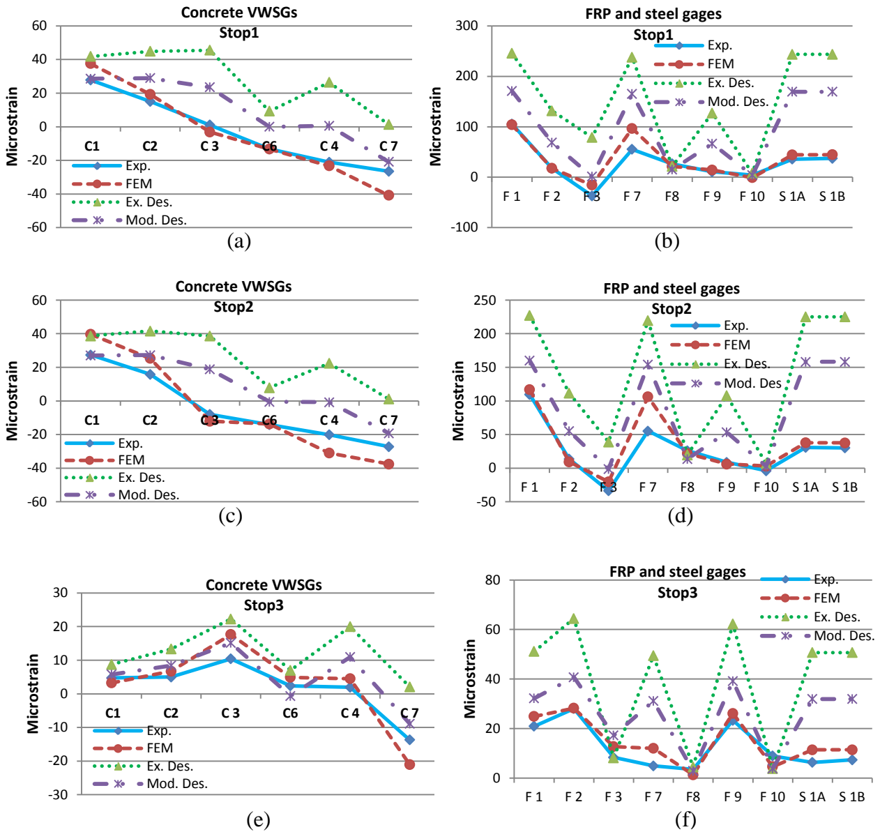
Figure 6-6 Strain Values in HCB2, B0410, Due to the Three Steps (Stage 3)
