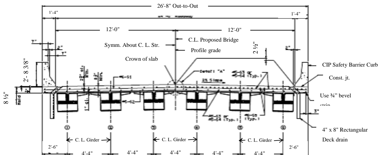
Figure 3-11 Typical Cross Section of Bridge B0478
