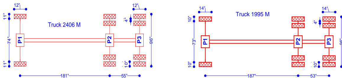
Figure 6-2 Truck Dimensions (B0410 Load Test)
