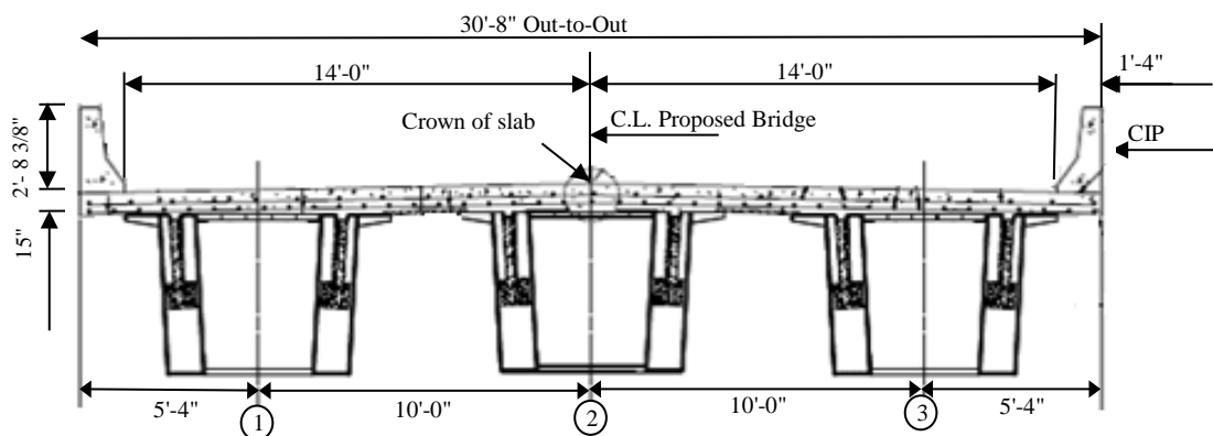
Figure 3-6 Typical Cross-Section of Bridge 0410
