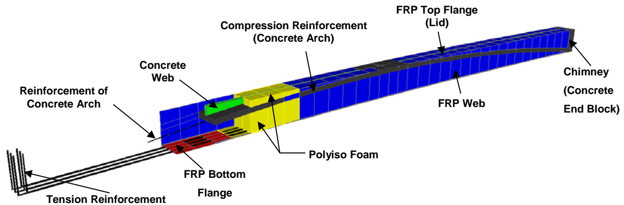
Figure 2-3 Fragmentary Perspective of Hybrid-Composite Beam
