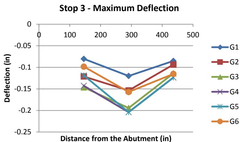
Figure 5-13 Measured deflections in B0478 girders due to Stop 3
