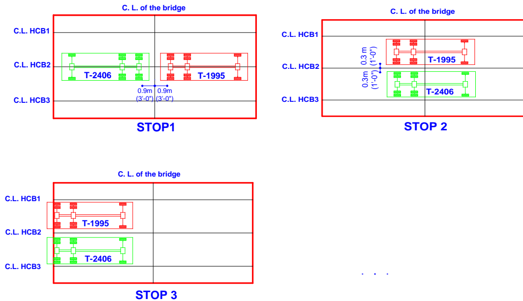
Figure 6-1 Truck Stops during B0410 Load Test
