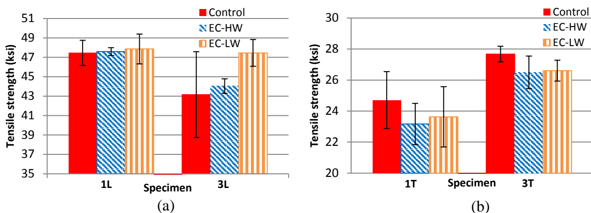
Figure 7-11 Tensile Strength of Control and EC Specimens
