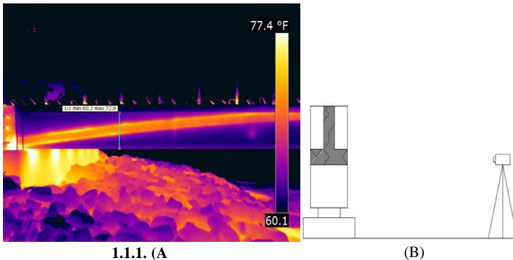
Figure 4-11: (A) Thermal Picture Perpendicular to HCB, (B) Diagram of Corresponding Camera Location Mockup Testing
