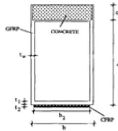
Figure 2-2 Hybrid FRP-Concrete Cross Section
