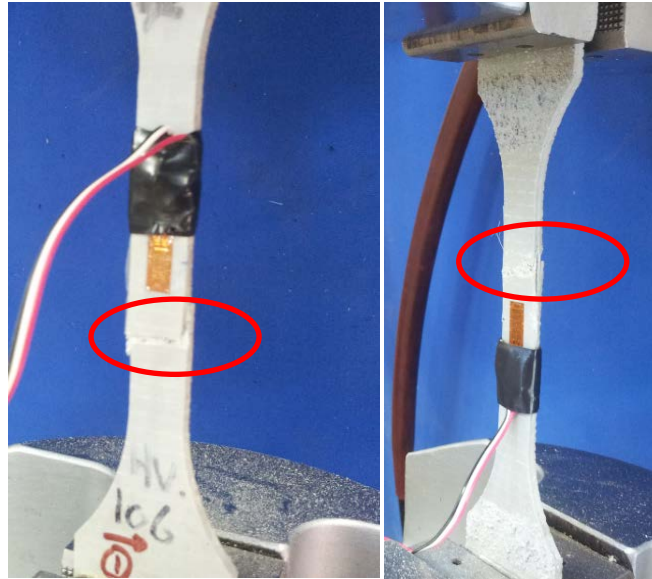
Figure 7-2 Failure Locations in Dumbbell-Shaped GFRP
