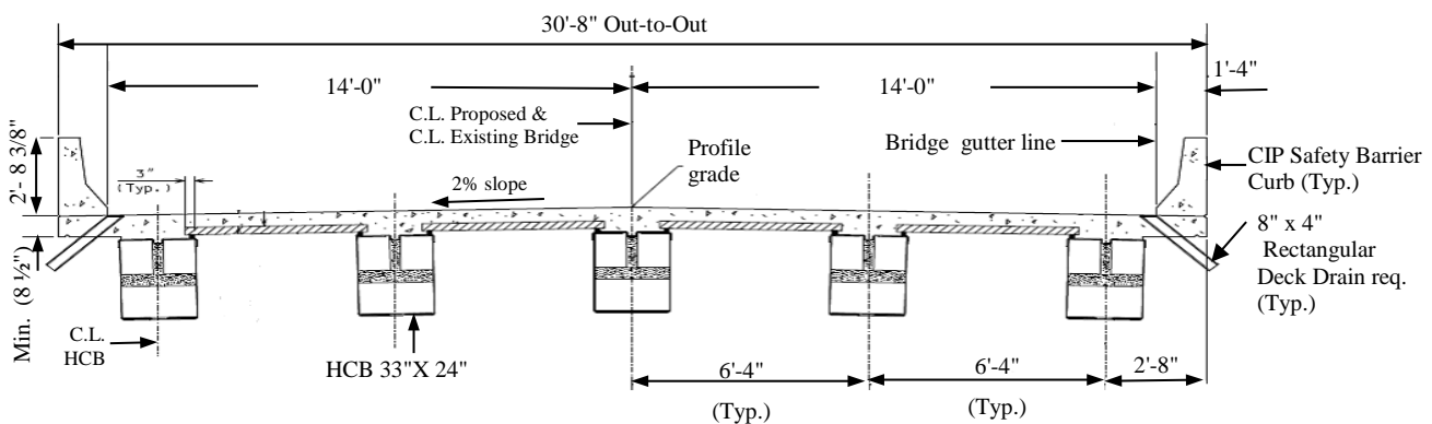
Figure 3-1 Bridge B0439 Typical Cross Section
