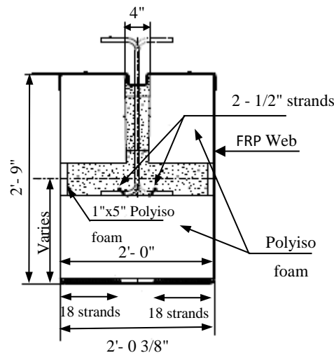
Figure 3-2 Typical Cross Section of B0439 HCB
