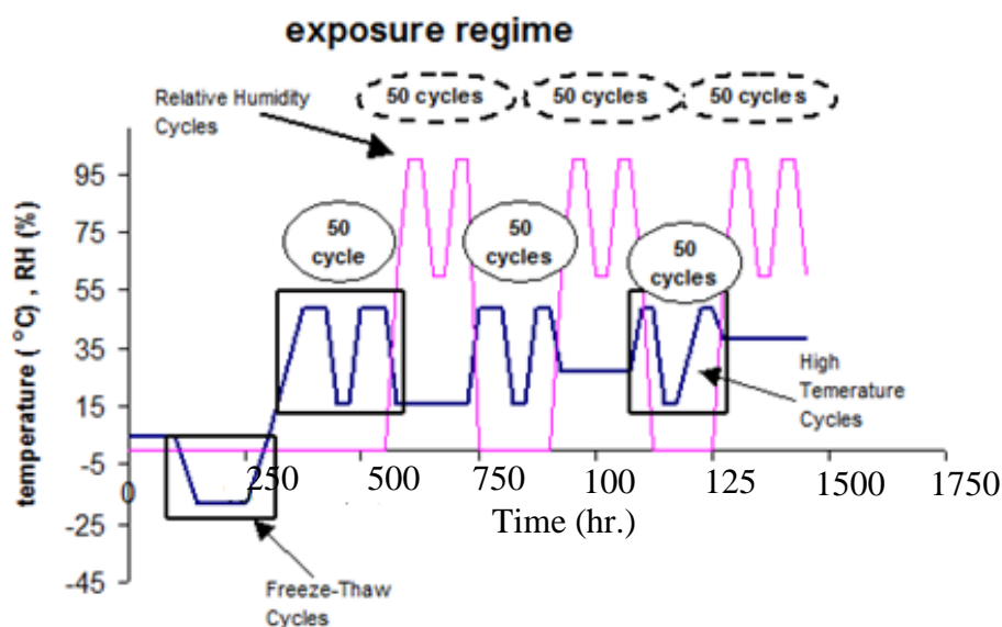
Figure 7-4 The Environmental Chamber Exposure Regime
