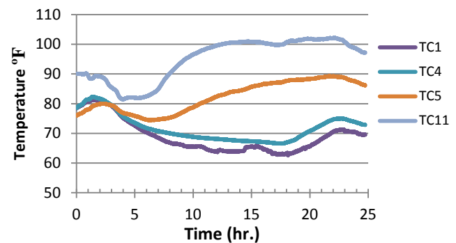
Figure 4-25 Strands Temperature of HCB2, B0410 during and after the Arch Pour
