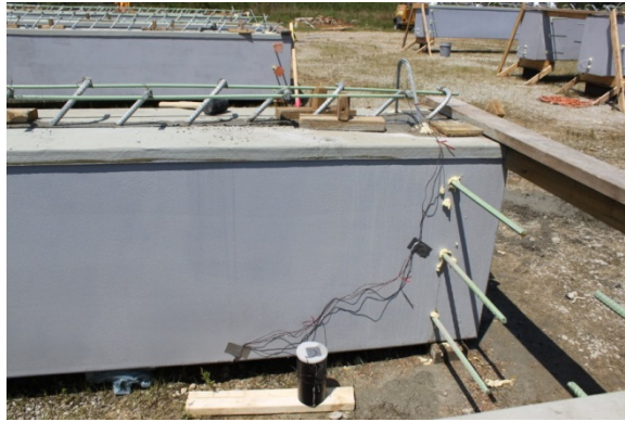
Figure 4-23 Overview of Maturity Meter Setup
