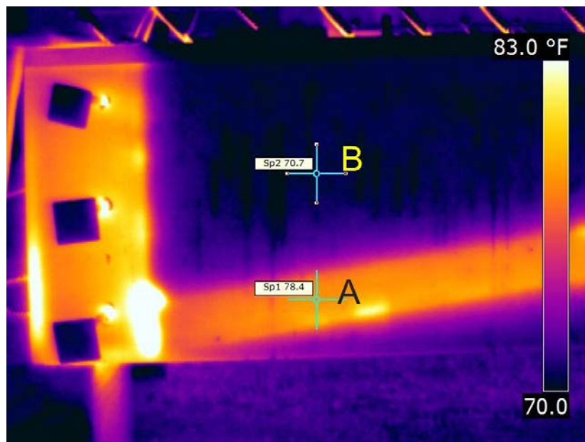
Figure 4-15 Figure illustrating how temperature contrast was determined.
