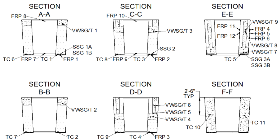
Figure 3-15 Instrumentation of HCB2, B0410 (Cross-Sections)
