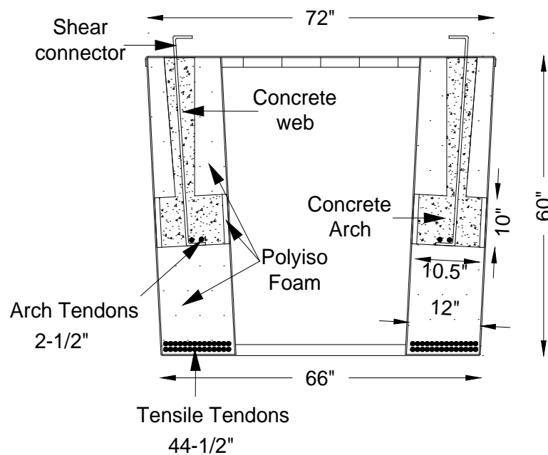
Figure 3-7 Typical Cross Section of B0410 HCB
