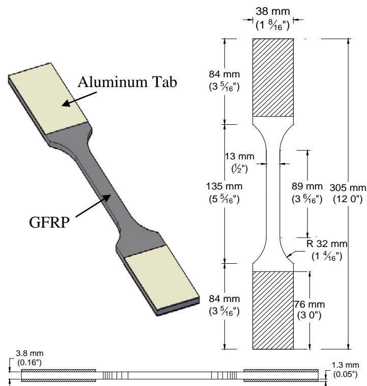
Figure 7-1 Dimension of FRP Specimens
