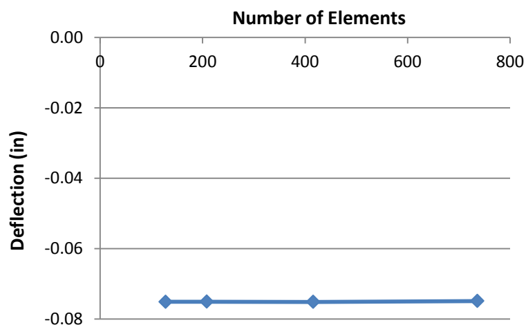
Figure 5-6 Deflection of HCB parabolic arch (Convergence Study)
